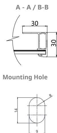
Frame Cross Section
